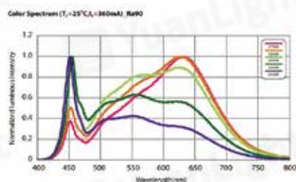
LED 光譜圖
